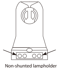
Non-shunted lampholder
