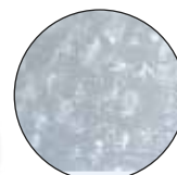
• 63478 Barkley 1 Light LED Wall Fixture Galvanized Steel Finish with Clear Seeded Glass Height: 11.89" Width: 6.06" Extends: 7.28" Height from Center of Outlet Box: 2.20" Back Plate: H: 5.11" W: 5.11" Includes 13 Watt Integrated LED
