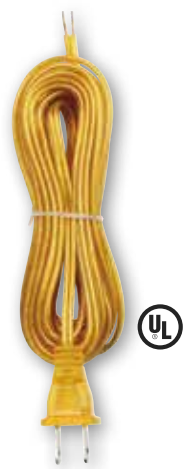
70103 15' Gold Cord Set Polarized Plug 18-2 SPT-1, 105° Wire
