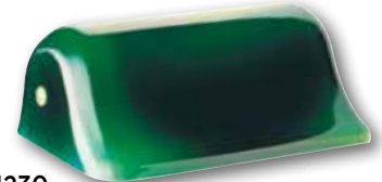
• 81230 Green with White Interior Glass Shade Height: 3.13" Width: 8.75" Depth: 5.00" 1/2" holes on both sides
