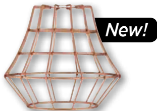
85085 Brushed Copper Angled Bell Cage Shade Fitter: 2.25" Height: 6.50" Diameter: 7.60"
