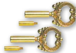
70160 Two Socket Keys Brass Finish With 1/2" Extensions Tapped 3/16-F x 1/16-M
