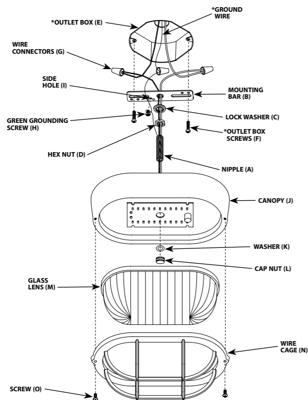
FIGURE 1. Line art shown may not exactly match the fixture enclosed. However, the installation instructions do apply to this fixture.
