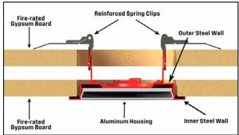
Representation of typical 2-hour fire-rated construction
