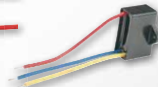
77091 Fan Capacitor 3 MFD and 6.5 MFD 3-Wire 150V
