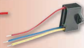
77091 Fan Capacitor 3 MFD and 6.5 MFD 3-Wire 150V
