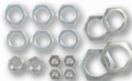
70152 Sixteen Assorted Hex Nuts Steel Includes: • 4 8-32 Hex Nuts • 2 \frac{1}{4} -27 Hex Nuts • 6 \frac{1}{8} -IP Hex Nuts • 2 \frac{1}{4} -IP Hex Nuts • 2 \frac{3}{8} -IP Hex Nuts
