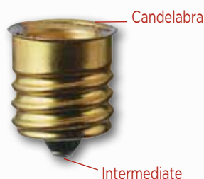
* 22403 Socket Adapter Reducer Reduces Intermediate Base to Candelabra Base With Rubber Ring 75 Watts Max. 120 Volts
