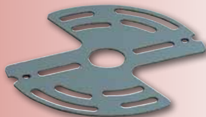
* 21030 Universal Crossbar Slips \frac{3}{8} -IP Can Be Used for Porch Bracket, Ceiling Fixture or Any Other Type of Wall Mounted Lamp Easily Adjustable for Slot Mounting Two No. 10 Wood Screw Holes Will Adjust on 3", 3 \frac{1}{4} " or 4" Box 35 lb. Load Rating
