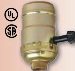
* 22051 - Polished Brass 2 Circuit Turn Knob Medium Base Bushing 1/8-IP with Set Screw Removable Knob 250 Watts Max., 250 Volts Height - 2 1/2"
