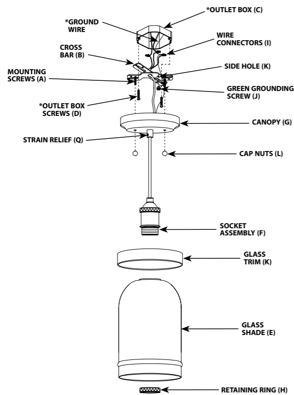
FIGURE 1. Line art shown may not exactly match the fixture enclosed. However, the installation instructions do apply to this fixture.
